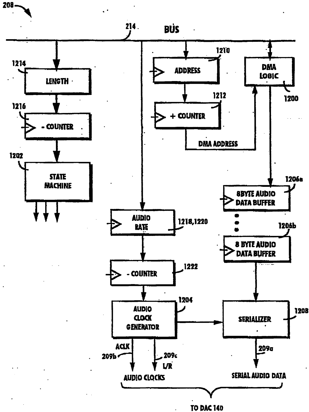
EXAMPLE AUDIO INTERFACE ARCHITECTURE
